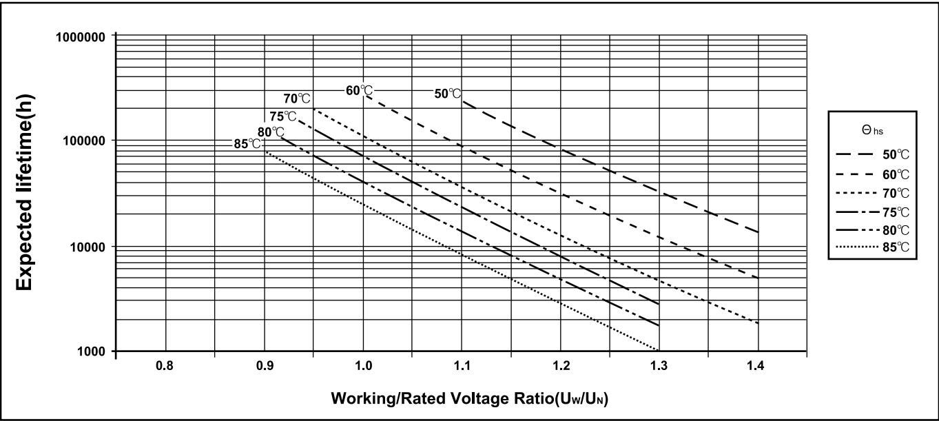
预期寿命曲线 Expected Lifetime curve
